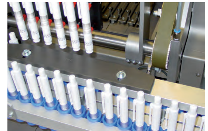
Pen Insertion Pens or Injectors are delivered standing upright through a PUCK system
